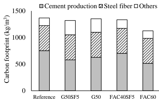
Figure 2.10. Carbon foot print results of the UHPC mixtures.
