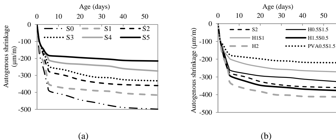
Figure 5.5 Autogenous shrinkage of: (a) mixtures with different fiber contents; (b) mixtures made with different fiber combinations.
