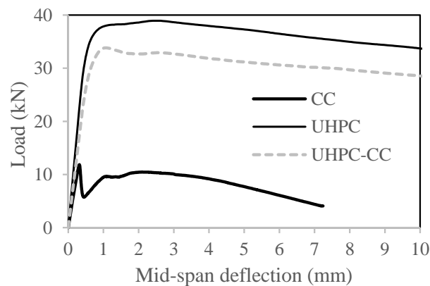
Figure 9.20. Load-deflection relationships.
