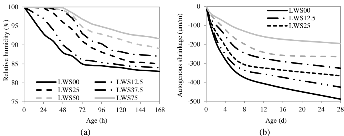
Figure 3.3. Experimental results of relative humidity and autogenous shrinkage: (a) IRH in the first 7 d and (b) autogenous shrinkage in the first 28 d.
