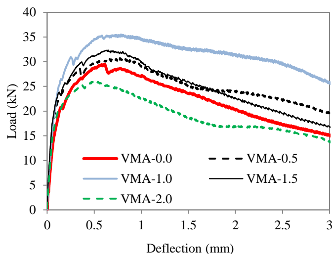
Figure 4.4. Load-deflection curves of UHPC-F mixtures with different VMA contents.
