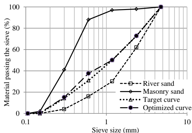
Figure 2.8. Sand gradations.
