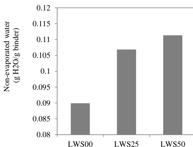
Figure 3.8. Non-evaporated water of investigated UHPC mixtures at 28 d.
